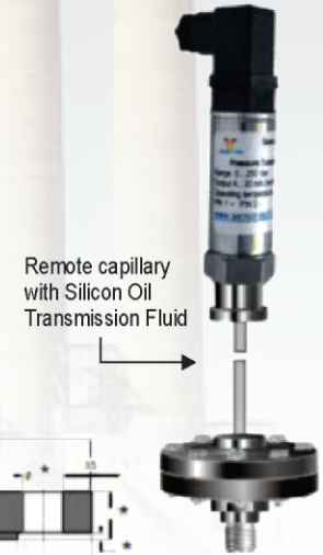
Diaphragm sealed end
