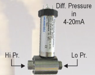
Differential PTx with Orifice plates / Venturi tubes
